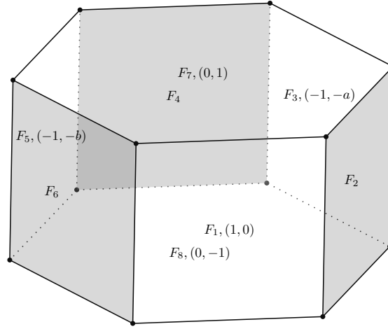
Fig. 1: Polytope Q with distinguished facets (gray) and isotropy function for n = 2 . F_1, \dots, F_6 are sides of Q counterclockwise and F_7, F_8 are top and bottom facets of Q , resp.
