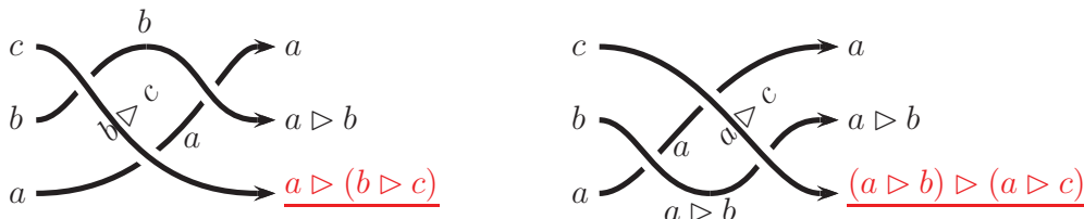
Figure 4: Reidemeister III move \iff self-distributivity
