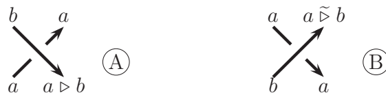
Figure 3: Coloring rules for positive and negative crossings
