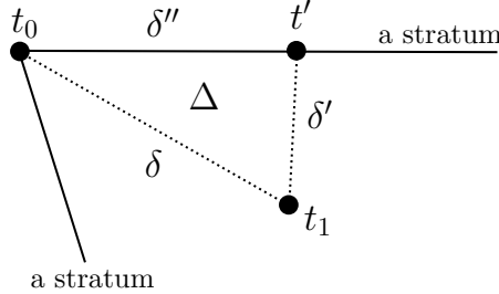
FIGURE 2. A triangle \Delta and s-arcs \delta , \delta' and \delta'' .
