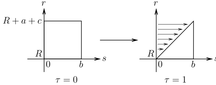
FIGURE 1. The homotopy \phi_\tau .
